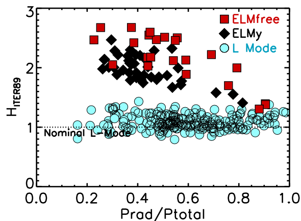
FIG. 39. Normalized energy confinement for the L-mode can be maintained, even at very low levels of conducted power. In contrast, the H-mode confinement deteriorates at a high radiated power because of the decrease in pedestal temperature. Reprinted with permission from Greenwald et al. , Nuclear Fusion 37 , 793 (1997). Copyright 1997 IOP. 17
