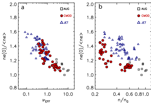
FIG. 43. Density peaking ratios in C-Mod is overlaid on data from AUG and JET showing that the appropriate scaling is collisionality (a) rather than n/n_G (b) thus implying a moderate level of peaking for ITER baseline discharges. Reprinted with permission from Greenwald et al. , Nuclear Fusion 47 , L26 (2007). Copyright 2007 IOP. 182
