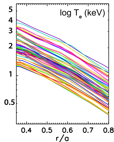
FIG. 38. Profile self-similarity is demonstrated. Te profiles are plotted, on a semi-log scale for a random selections of shots and time including the OH, L-mode, and H-modes at a wide range in density and input power. Greenwald et al. , Fusion Sci. Tech. 51 , 266 (2007). Copyright 2007 American Nuclear Society. 185
